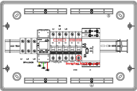
Horizontal-mounted: Single-phase single inverter
