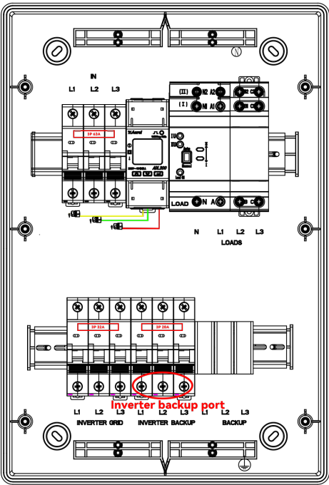
Vertical-mounted: Three-phase inverter
