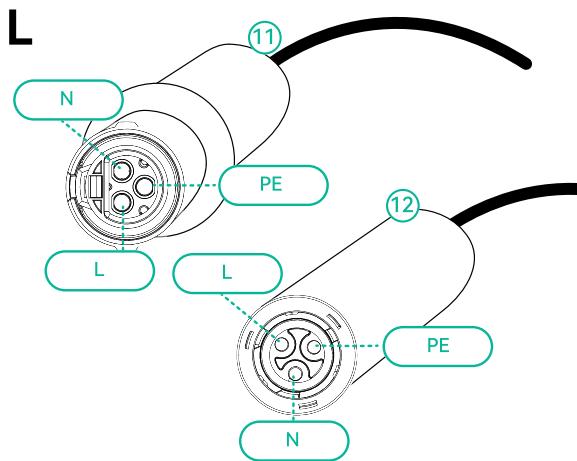
Wire AC cables (use 6-10mm 2 outdoor cables )
