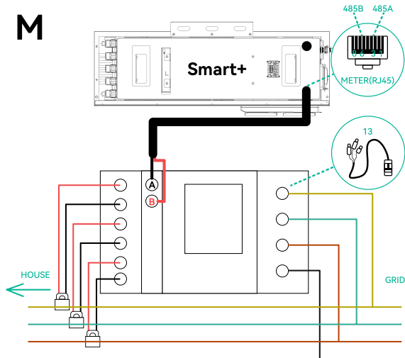
Wire the Meter & CT's ( All CT Arrows should point towards the house )
