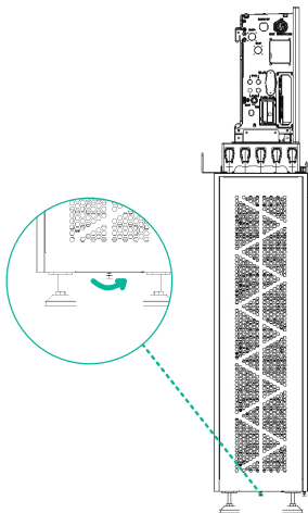
Apply and secure the Battery House Side Panel
