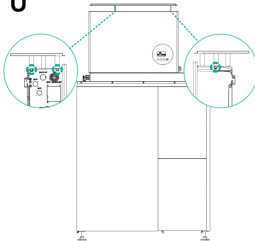
Install and secure the Enclosures
