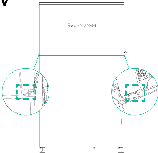
Apply and secure the Battery House Side Panel
